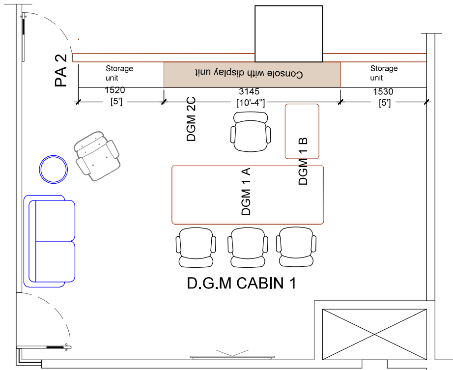
Plan
